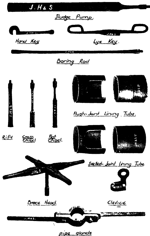
Fig. 12.—Hand Boring Tools.
